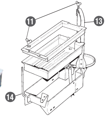
Battery Casing and Air Cleaner Support, Series II, IIA, III, 2.25 petrol
