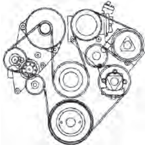
Discovery II Serpentine Belt Layout, with ACE
